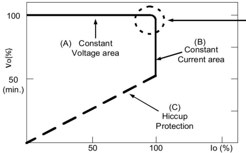
Typical LED power supply I-V curve
